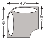
44141 CORNER WEDGE
